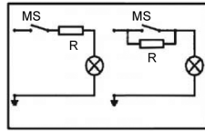
Fig. 2: Lamp load provided with resistance in parallel or series connection to switch of condensers
